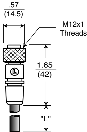
STRAIGHT FEMALE RKT
