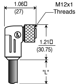
RIGHT ANGLE FEMALE RKWT
