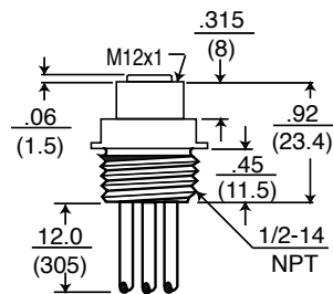
FEMALE RECEPTACLE w/ 1/2 NPT
