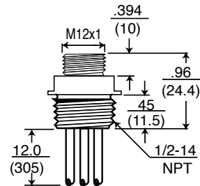
MALE RECEPTACLE w/ 1/2 NPT
