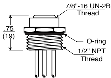
FEMALE RECEPTACLE RKF
