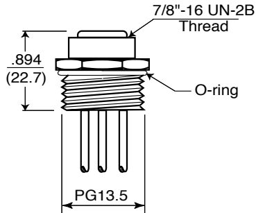
FEMALE RECEPTACLE RKF
