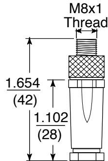
ATTACHABLE MALE CONNECTOR RSMC
