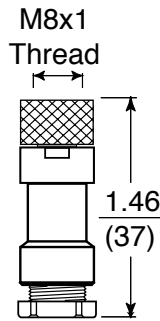
ATTACHABLE FEMALE CONNECTOR RKMC
