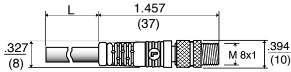
STRAIGHT MALE LOCKING PLUG RSMV
