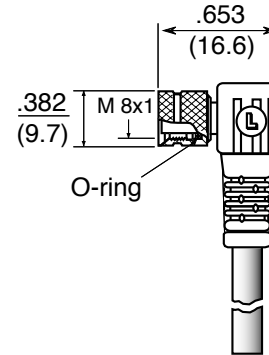
RIGHT ANGLE FEMALE LOCKING PLUG RKMWW
