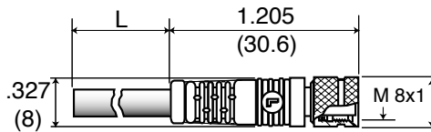
STRAIGHT FEMALE LOCKING PLUG RKMV
